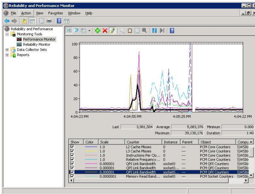
Windows* Perfmon
